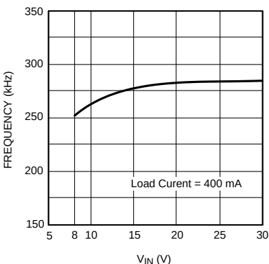
Figure 16. Frequency vs V_{IN} Circuit of Figure 14
